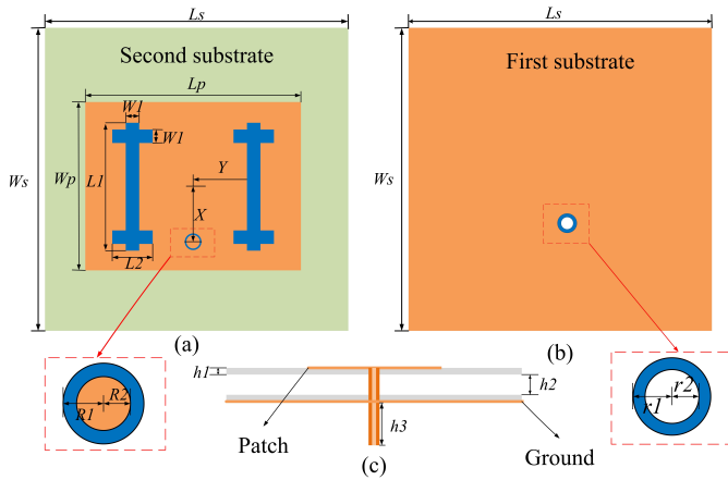
Fig. 3. Configuration of the antenna.(a) Top view. (b) Bottom view. (c) Side view. ( L_s = 52 , W_s = 52 , L_p = 26 , W_1 = 0.65 , X = 5.2 , R_1 = 1.43 , R_2 = 1.3 , r_1 = 0.74 , r_2 = 0.32 , h_1 = 0.508 , h_2 = 1.71 , h_3 = 3.9 , unit: mm)
