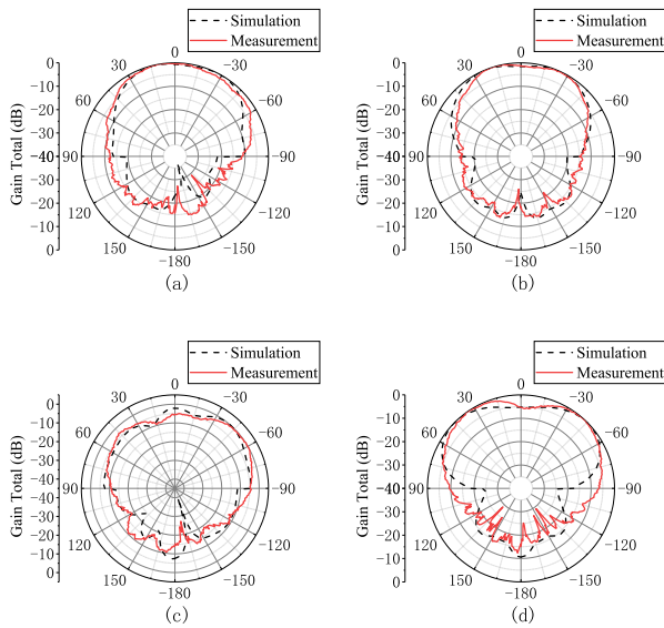
Fig. 11. Simulated and measured radiation patterns of Antenna 3.(a) 10.5 GHz (xoz-plane). (b) 10.5 GHz (yoz-plane). (c) 11 GHz (xoz-plane). (d) 11 GHz (yoz-plane).
