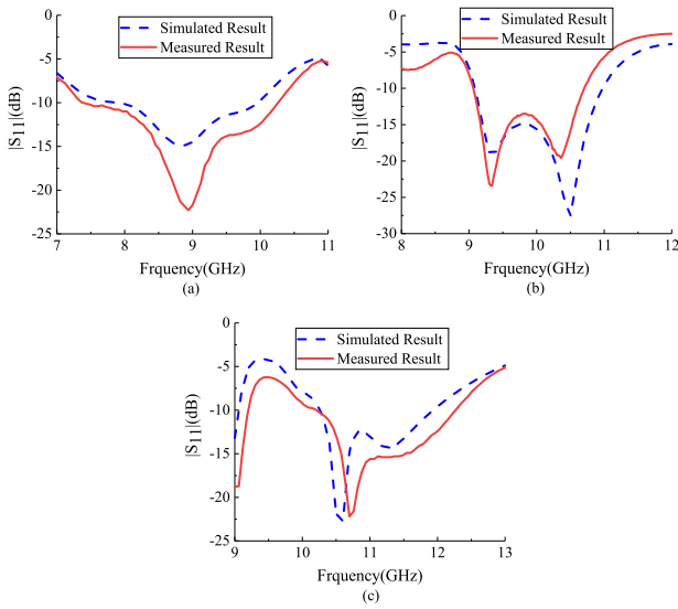
Fig. 8. Simulated and measured |S_{11}| of (a) Antenna 1, (b) Antenna 2 and (c) Antenna 3.
