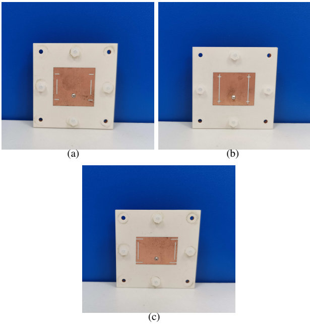
Fig. 7. The photos of (a) Antenna 1, (b) Antenna 2 and (c) Antenna 3.
