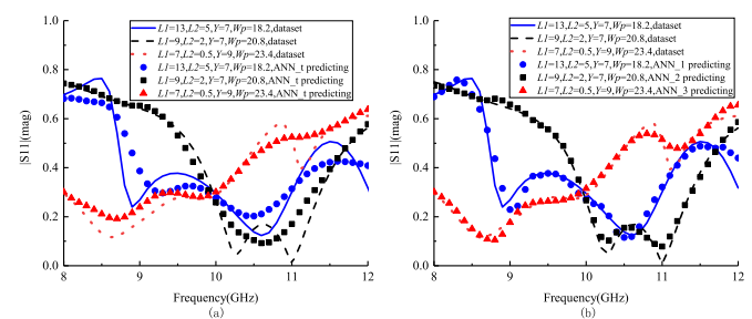
Fig. 4. The results of (a) ANN_t and of (b) ANN_1, ANN_2, ANN_3. Unit:mm.
