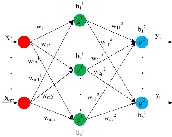
Fig. 1. The ANN with the input layer, one hidden layer and the output layer.
