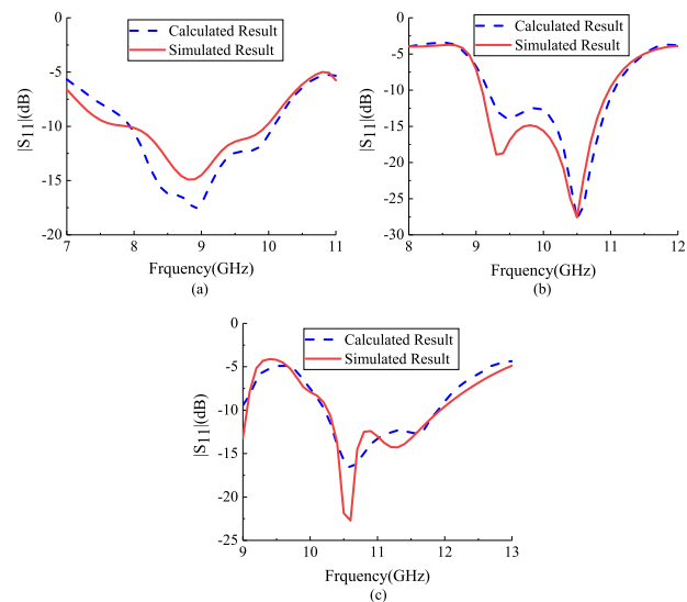
Fig. 6. Calculated and simulated |S_{11}| of (a) Antenna 1, (b) Antenna 2 and (c) Antenna 3.
