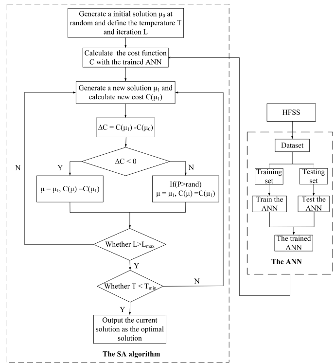
Fig. 2. Flow chart of the proposed hybrid method.
